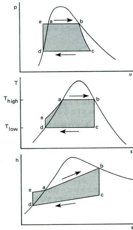
Figure 25.11 Basic Rankine Property Plots
