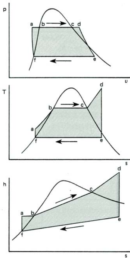
Figure 25.13 Rankine Cycle with Superheat
