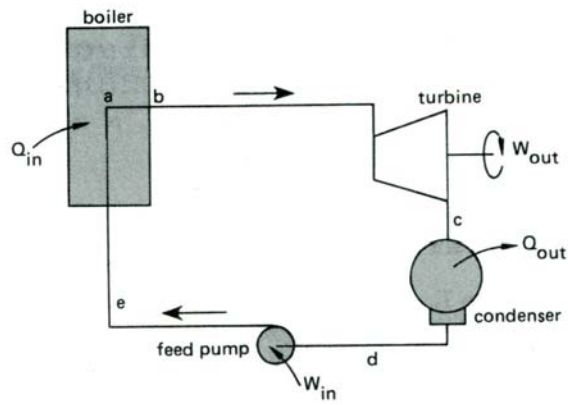
Figure 25.10 Basic Rankine Cycle
