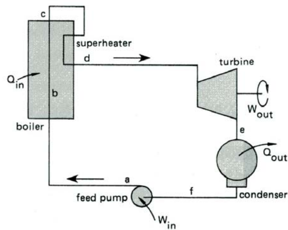
Figure 25.12 Rankine Cycle with Superheat
